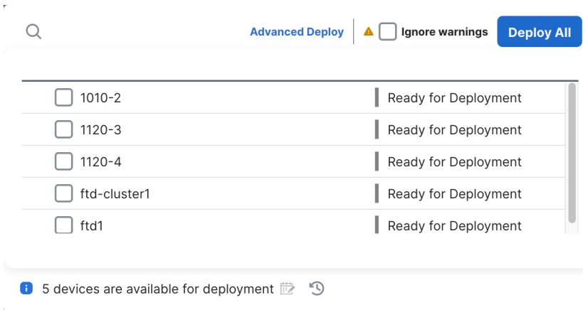
Figure 42: Deploy All
