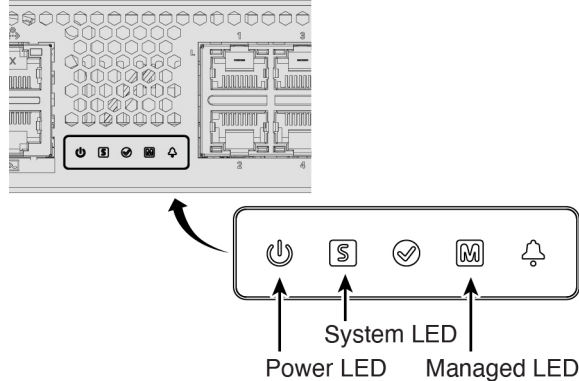
Figure 2: LEDs
