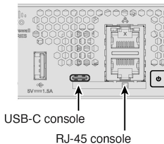
Figure 3: Console Port
