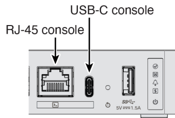
Figure 3: Console Port
