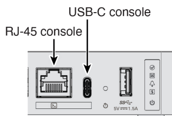
Figure 8: Console Port
