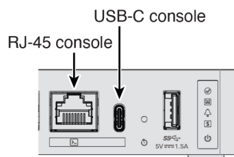
Figure 4: Console Port
