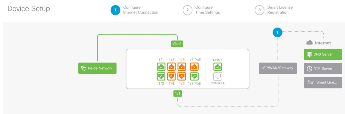
Figure 1: Device Setup
