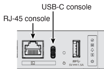
Figure 3: Console Port
