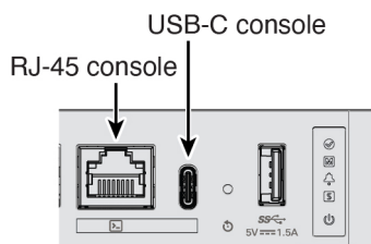
Figure 8: Console Port
