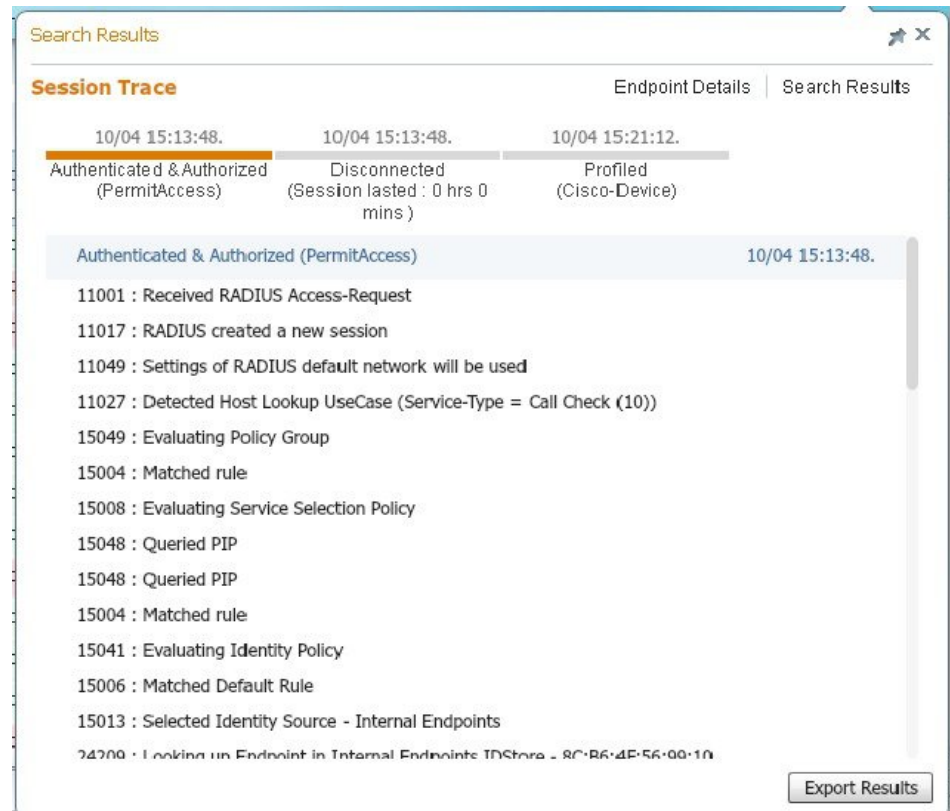
Figure 15: Session Trace of an Endpoint
