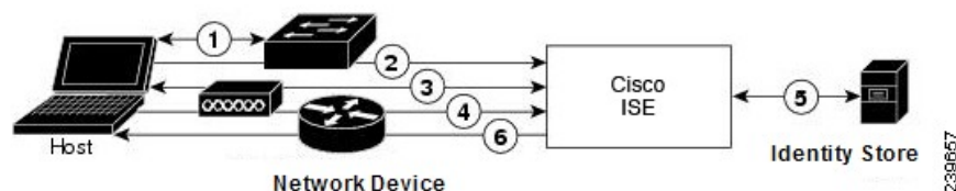
Figure 7: RADIUS-Based Authentication Without EAP
