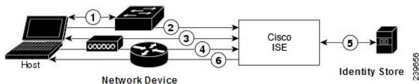
Figure 8: RADIUS-Based Authentication with EAP
