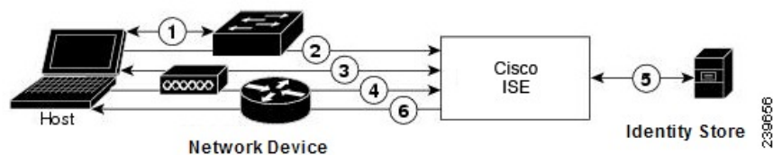
Figure 2: RADIUS-Based Authentication with EAP
