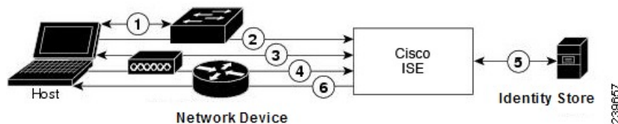
Figure 1: RADIUS-Based Authentication Without EAP
