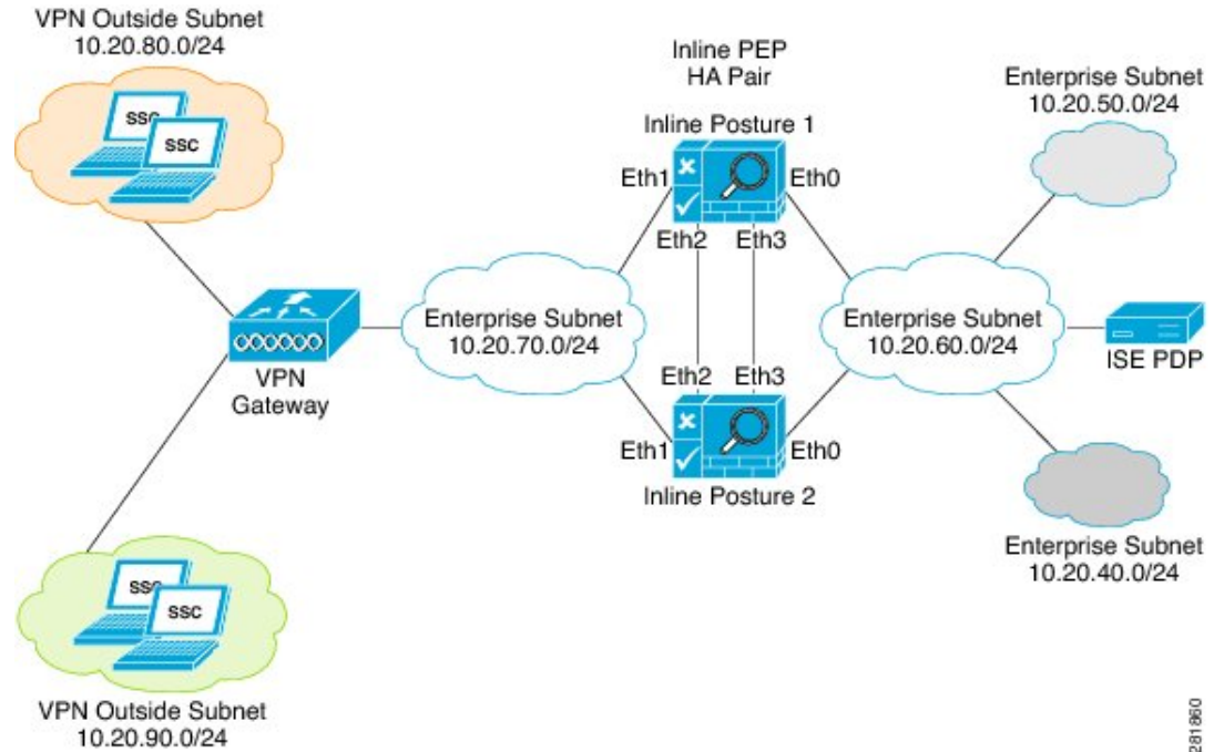
Figure 7: Inline Posture High-Availability Routed Mode Configuration
