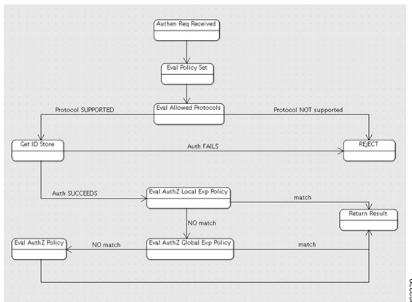
Figure 27: Policy Set Authentication and Authorization Evaluation Flow
