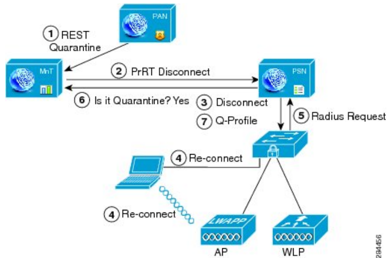
Figure 14: EPS Quarantine Flow
