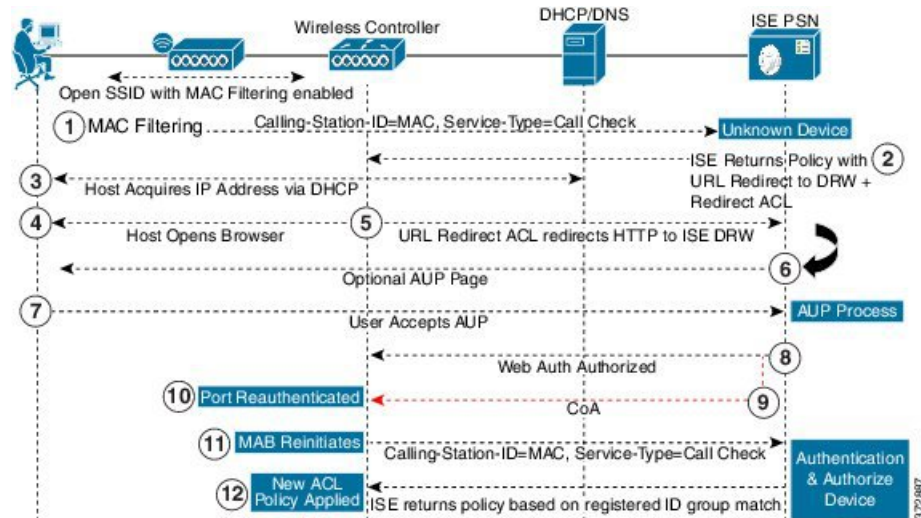
Figure 18: Wireless Device Registration Web Authentication Flow
