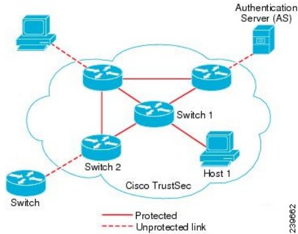
Figure 30: TrustSec Architecture
