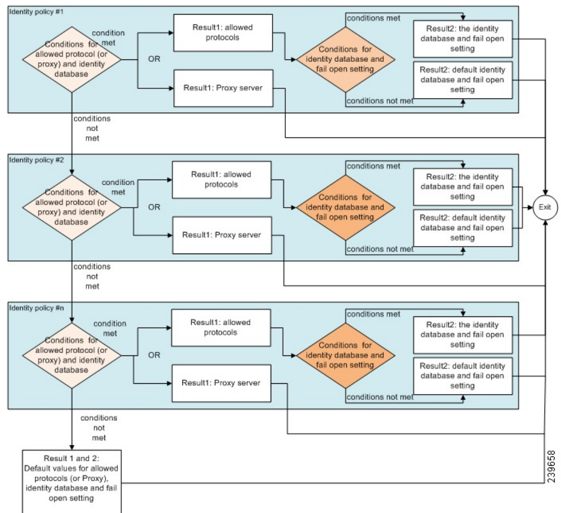
Figure 24: Rule-Based Authentication Policy Flow
