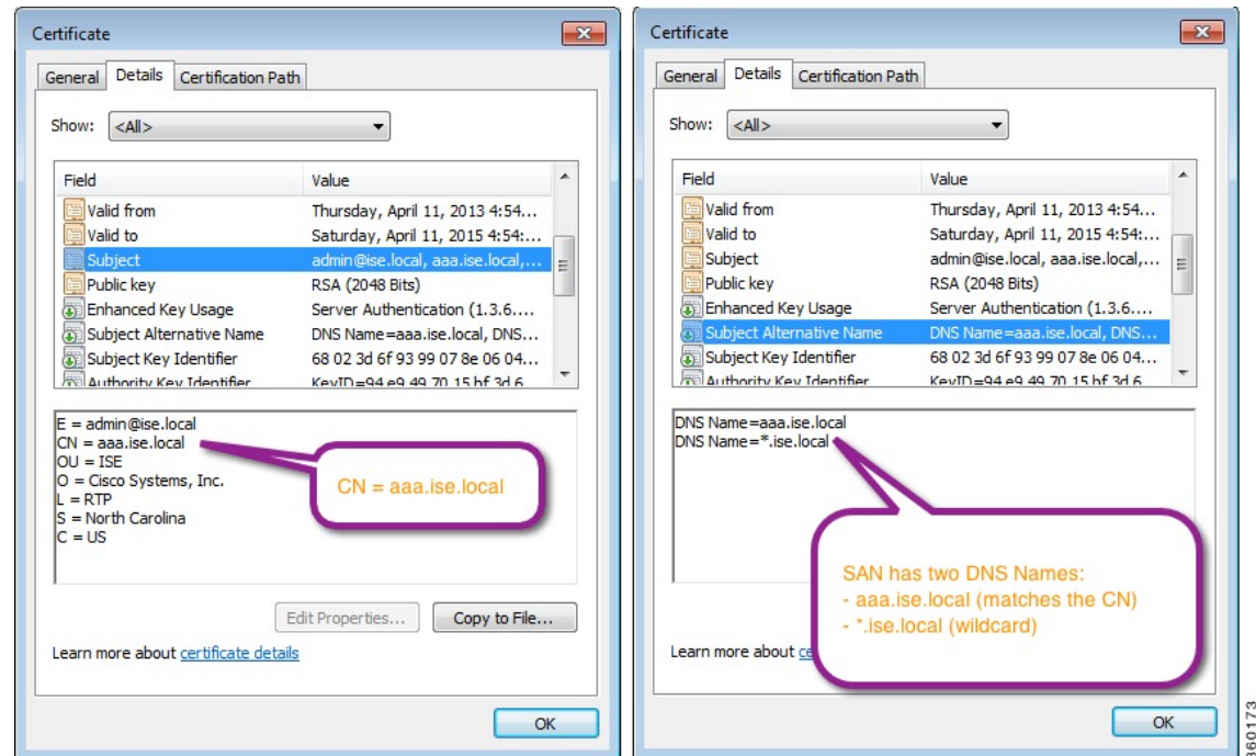
Figure 10: Wildcard Certificate Example
