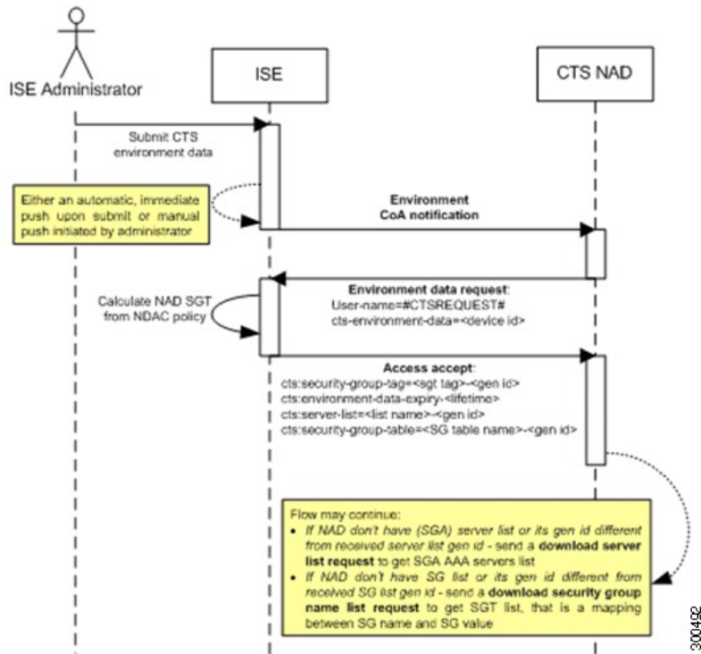
Figure 31: Environment CoA Notification Flow
