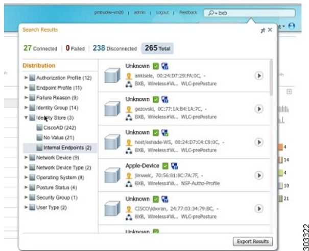
Figure 35: Search Result For Endpoints
