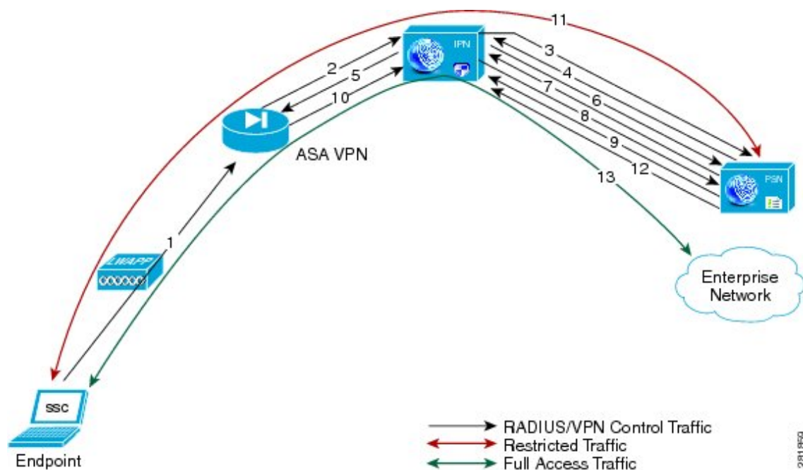
Figure 4: Inline Posture Policy Enforcement Flow
