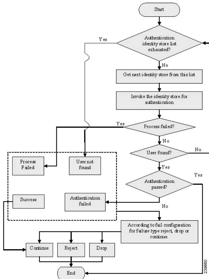
Figure 23: Simple Authentication Policy Flow
