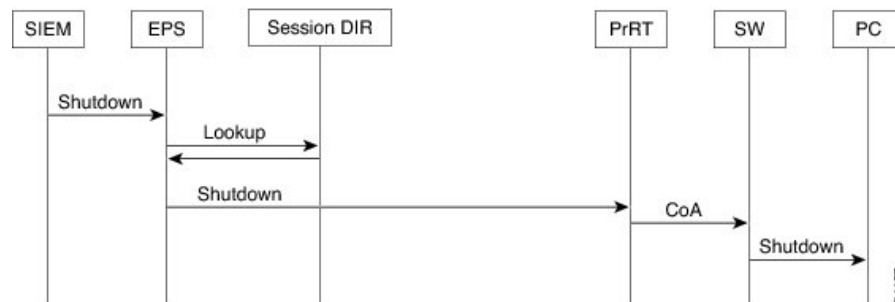
Figure 15: EPS Shutdown Flow
