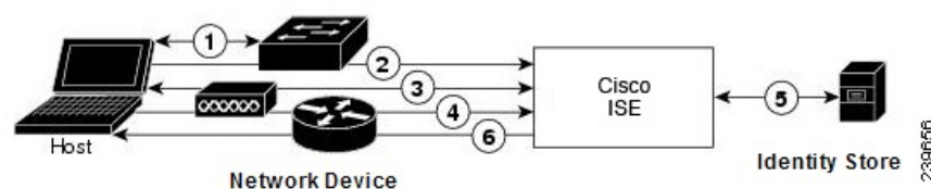
Figure 40: RADIUS-Based Authentication with EAP
