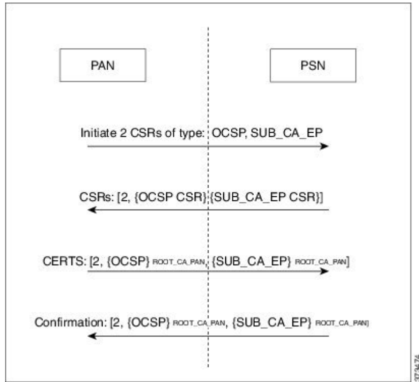
Figure 11: Certificates Provisioned At Node Registration - PSNs get an Endpoint CA and an OCSP certificates from the PAN
