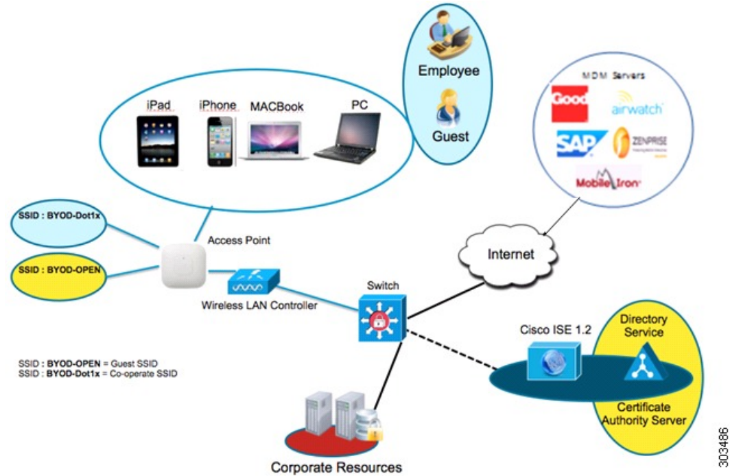
Figure 12: MDM Interoperability with Cisco ISE
