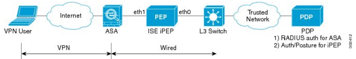
Figure 9: Cisco ISE Deployment with Inline Posture Node
