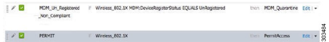
Figure 13: Authorization Policy Rules for the MDM Use Cases
