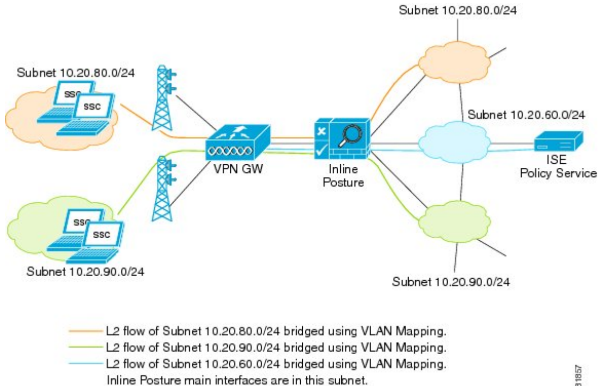
Figure 6: Inline Posture Bridged Mode Configuration
