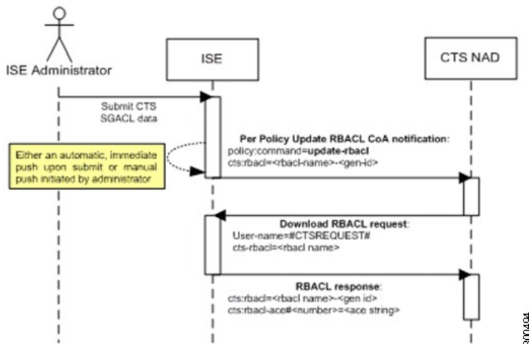
Figure 32: Update SGACL Content Flow
