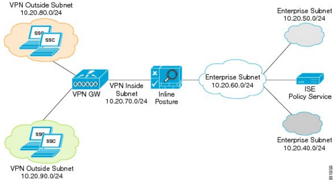
Figure 5: Inline Posture Routed Mode Configuration
