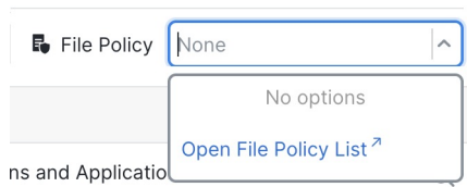
Figure 39: File Policy
