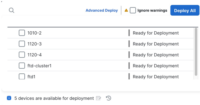
Figure 42: Deploy All
