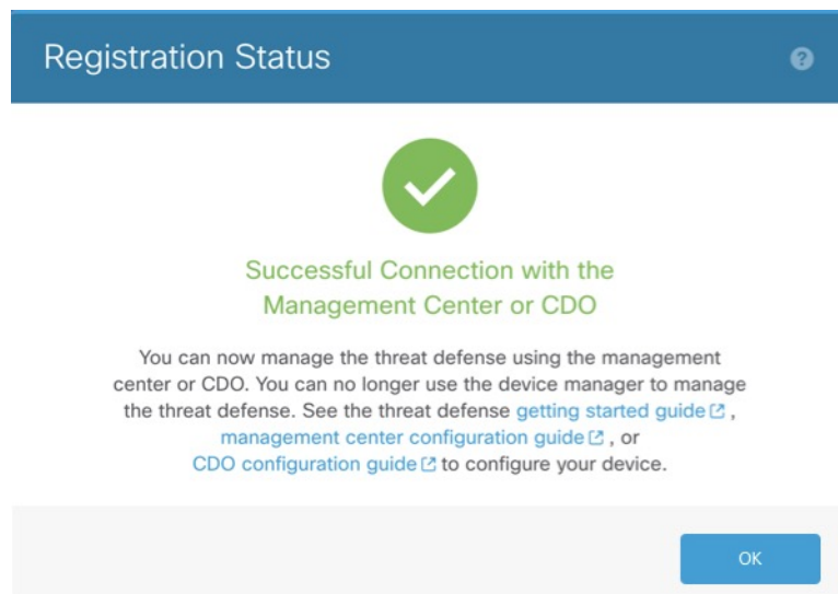
Figure 14: Successful Connection
