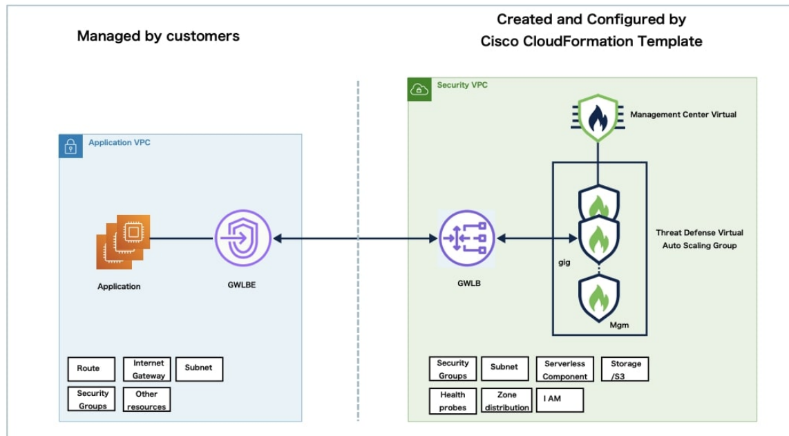
Figure 4: Firewall Threat Defense Virtual Auto Scale Solution with GWLB
