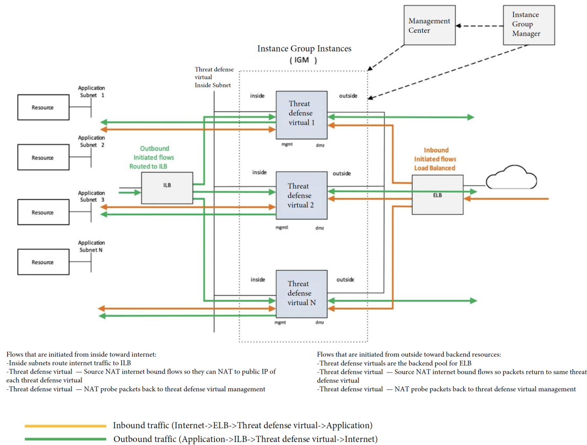
Figure 43: Firewall Threat Defense Virtual Auto Scale Use Case
