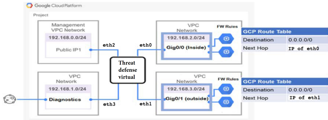
Figure 42: Sample Firewall Threat Defense Virtual on GCP Deployment
