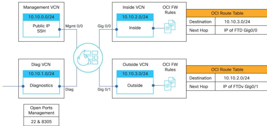
Figure 2: Sample Firewall Threat Defense Virtual on OCI Deployment with four subnets in a VCN
