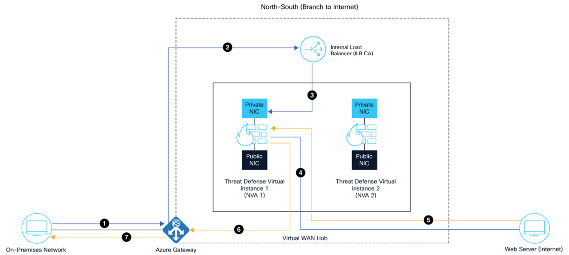
Figure 34: Firewall Threat Defense Virtual North-South Traffic Inspection Topology in Azure Virtual WAN Hub
