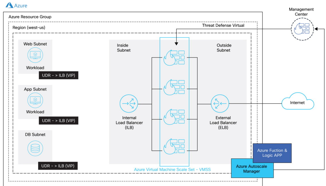
Figure 5: Firewall Threat Defense Virtual Auto Scale using Sandwich Topology Use Case Diagram
