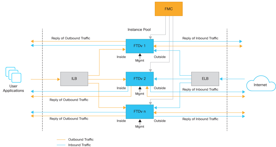
Figure 39: Secure Firewall Threat Defense Virtual Auto Scale Use Case Diagram
