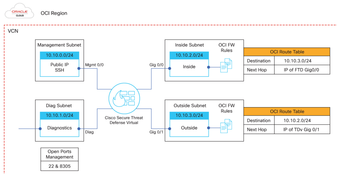
Figure 37: Sample Firewall Threat Defense Virtual on OCI Deployment with four subnets in a VCN
