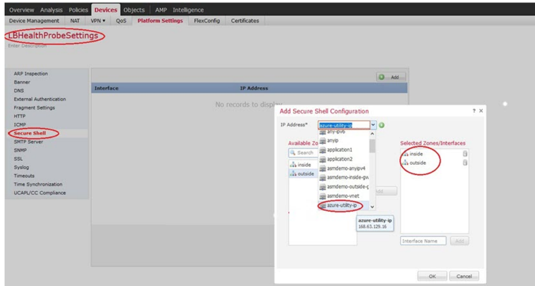
Figure 11: SSH Access for the Firewall Threat Defense Virtual Auto Scale
