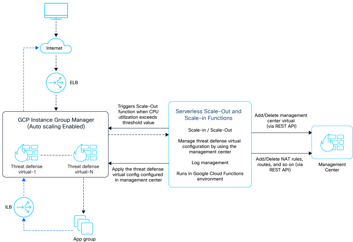
Figure 48: Auto Scale Solution Overview
