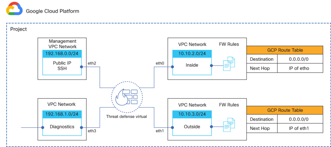
Figure 44: Sample Firewall Threat Defense Virtual on GCP Deployment
