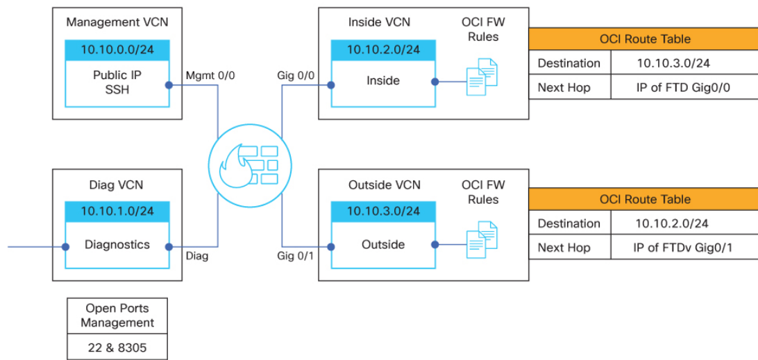
Figure 37: Sample Firewall Threat Defense Virtual on OCI Deployment with four subnets in a VCN
