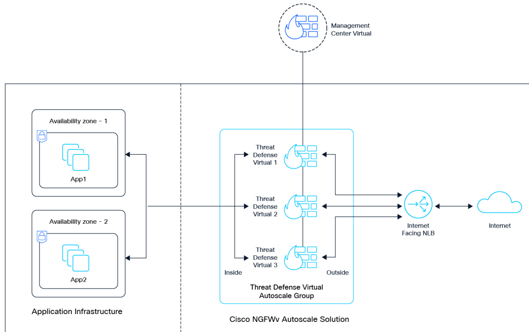
Figure 3: Firewall Threat Defense Virtual Auto Scale Solution with NLB
