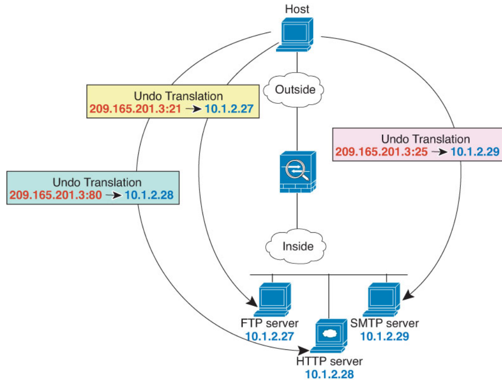
Figure 14: Static NAT-with-Port-Translation
