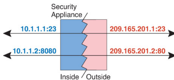
Figure 7: Typical Static NAT with Port Translation Scenario
