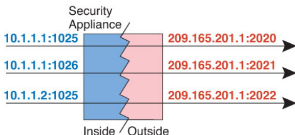
Figure 6: Dynamic PAT
