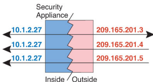
Figure 8: One-to-Many Static NAT
