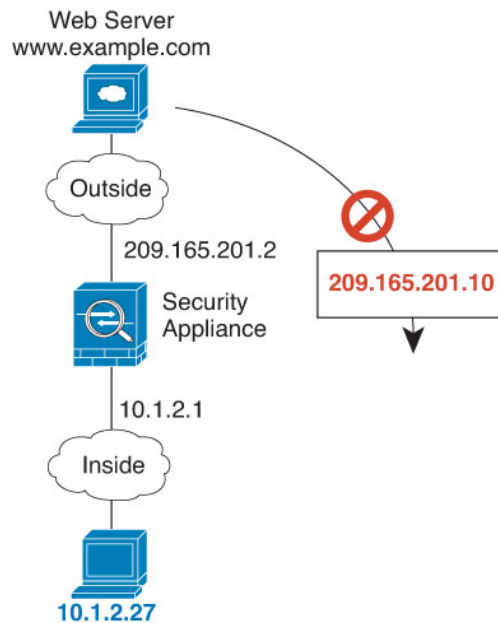
Figure 4: Remote Host Attempts to Initiate a Connection to a Mapped Address
