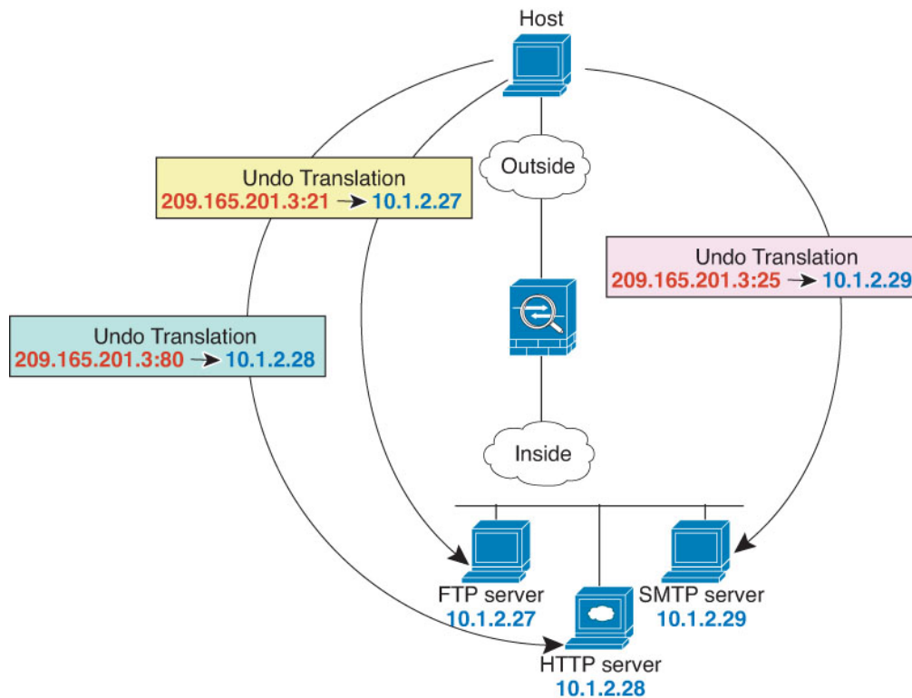
Figure 14: Static NAT-with-Port-Translation
