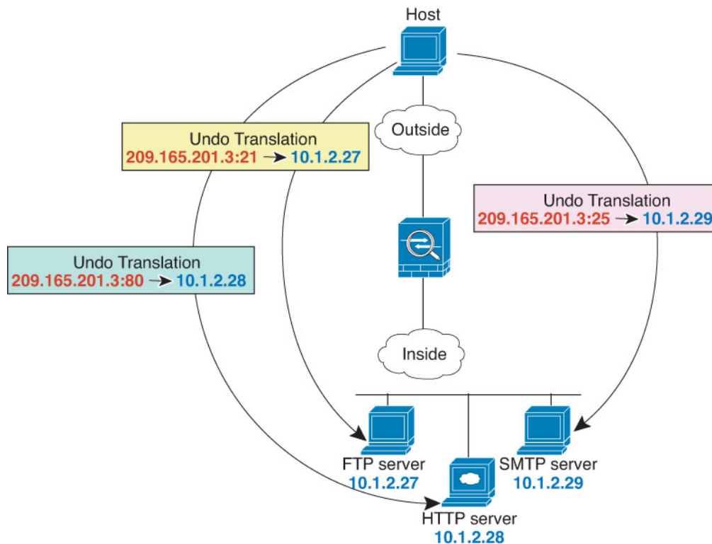
Figure 43: Static NAT-with-Port-Translation
