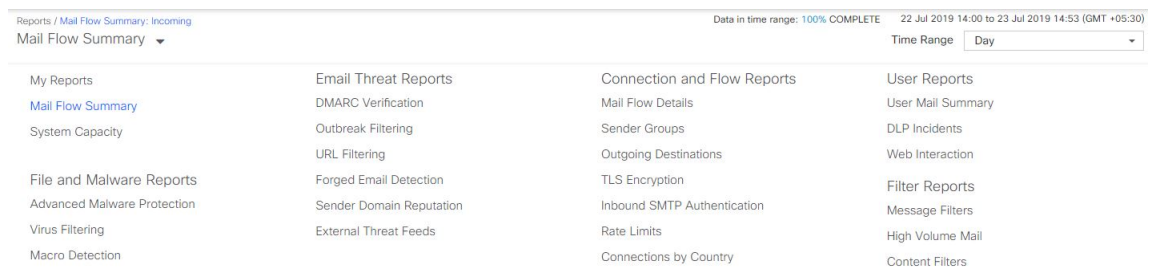
Figure 1: Reports Drop-down
