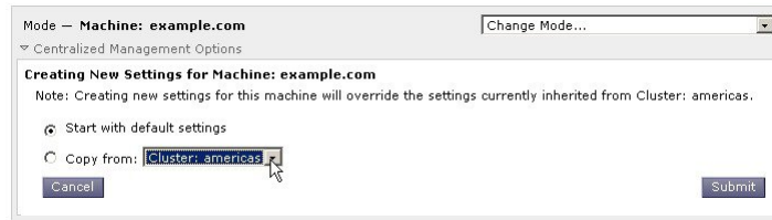
Figure 3: Centralized Management Feature in the GUI: Create New Settings
