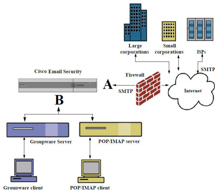
Figure 4: Public and Private Listeners for an Enterprise Gateway
