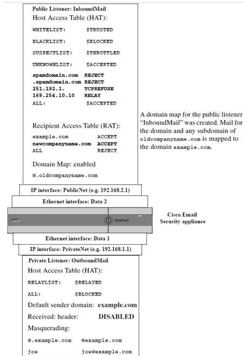
Figure 4: Domain Map Defined for a Public Listener
