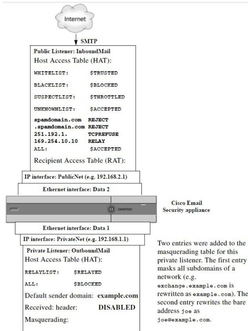
Figure 3: Masquerading Defined for a Private Listener
