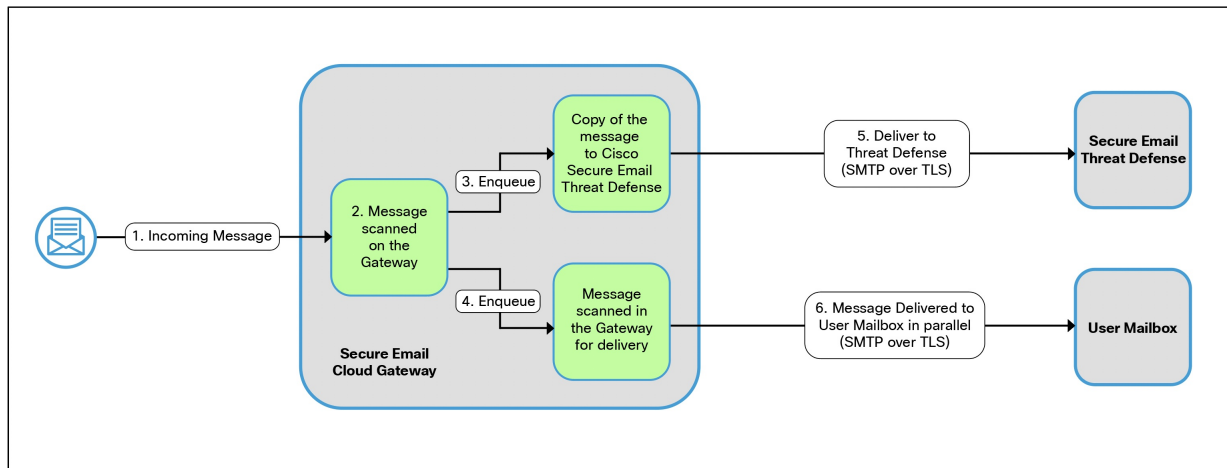
Figure 18: Overview of Threat Defense Connctor
