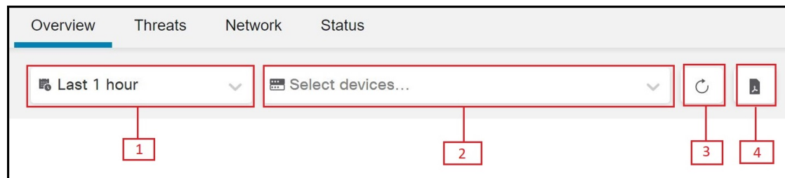
Figure 1: FTD Dashboard
