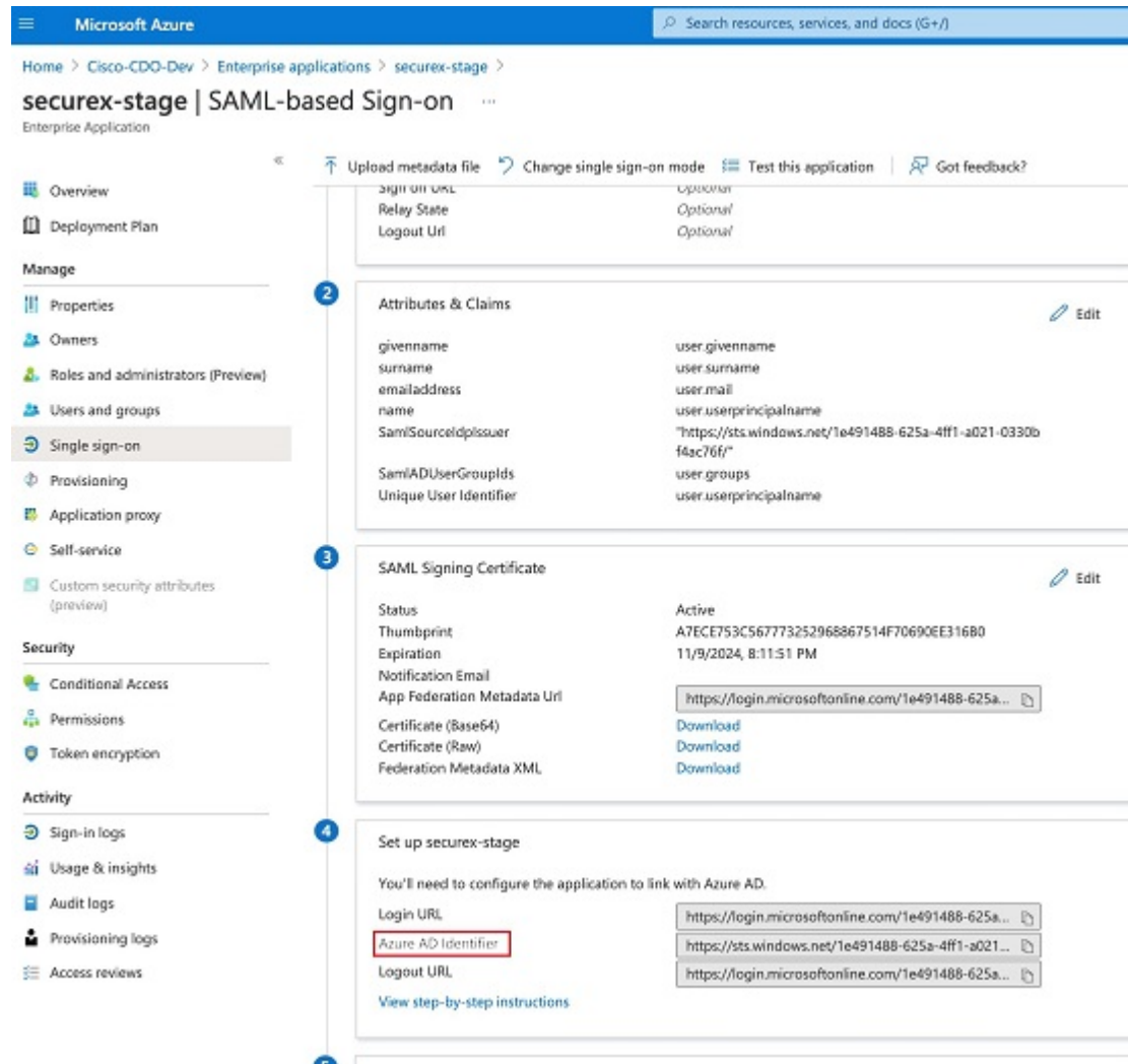
Figure 3: Locate the Azure Active Directory Identifier
