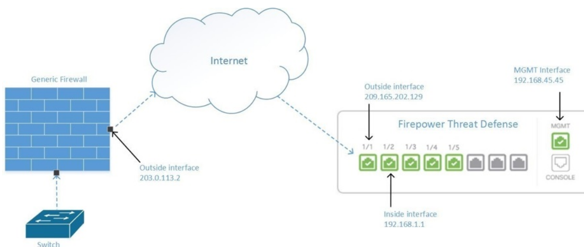
Figure 2: Device Management on Outside Interface
