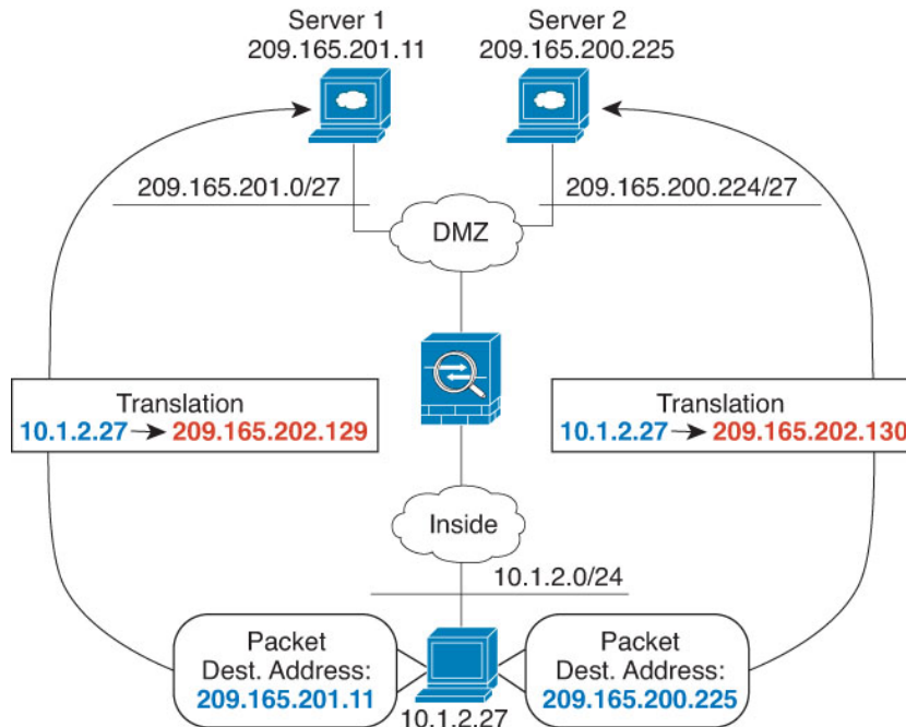
Figure 18: Manual NAT with Different Destination Addresses
