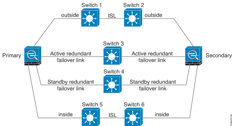
Figure 6: Connecting with Redundant Interfaces
