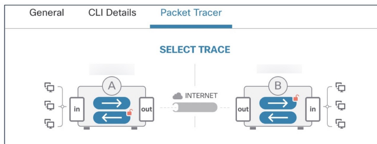
Figure 2: Packet Tracer
