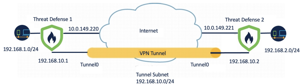
Figure 1: Static VTI VPN topology
