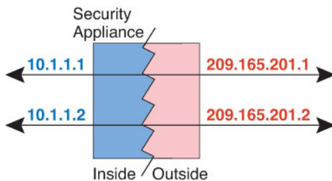
Figure 8: Static NAT
