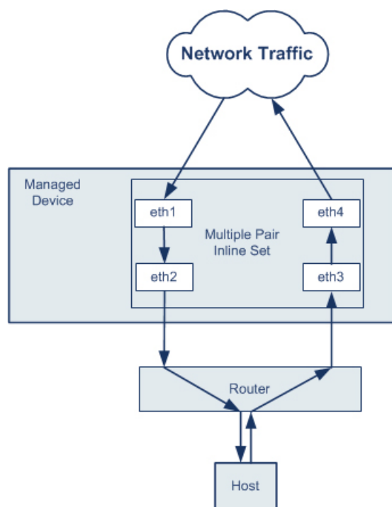
Figure 1: Asynchronous Routing
