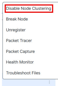
Figure 24: Disable Clustering
