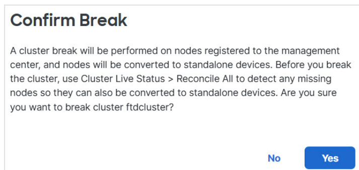
Figure 23: Confirm Break
