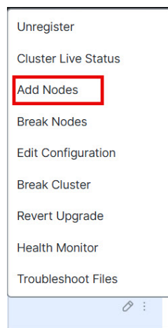
Figure 17: Add Nodes
