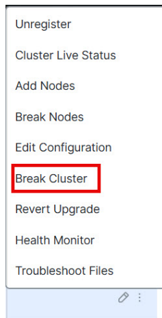
Figure 22: Break Cluster
