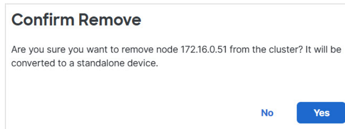
Figure 21: Confirm Break
