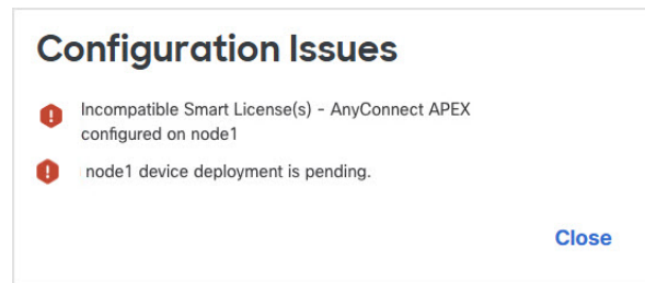
Figure 4: Configuration Issues
