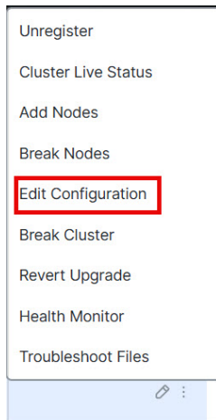
Figure 26: Edit Configuration
