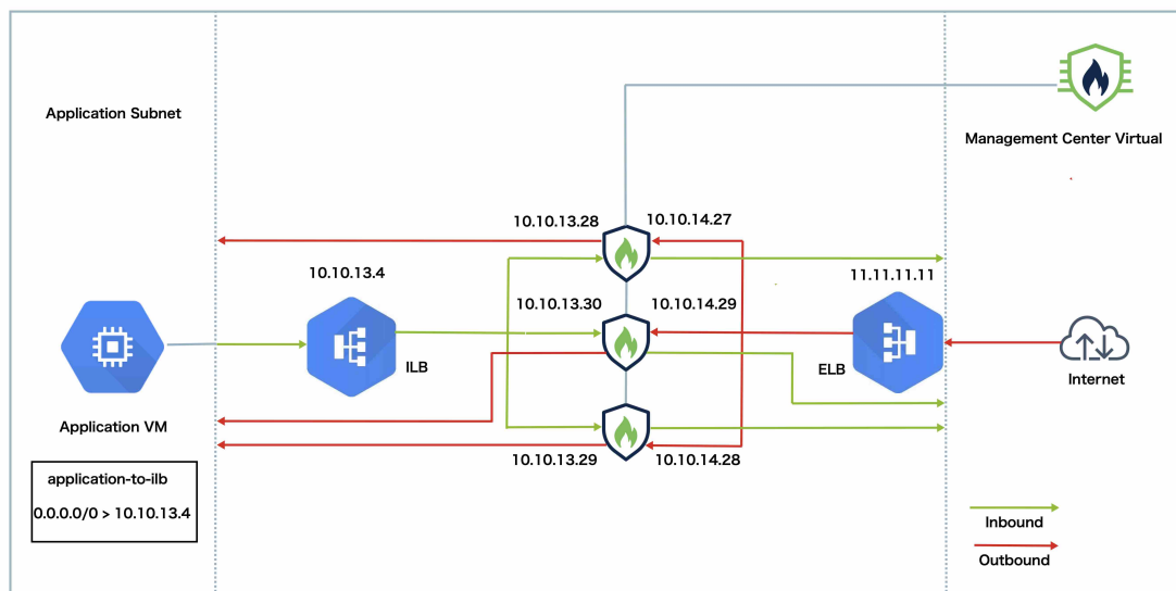
Figure 15: Sample Topology
