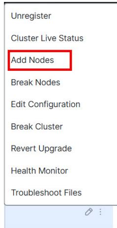
Figure 12: Add Nodes
