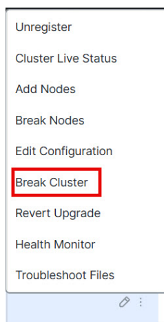
Figure 17: Break Cluster
