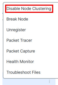
Figure 19: Disable Clustering
