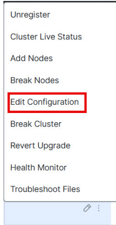
Figure 21: Edit Configuration
