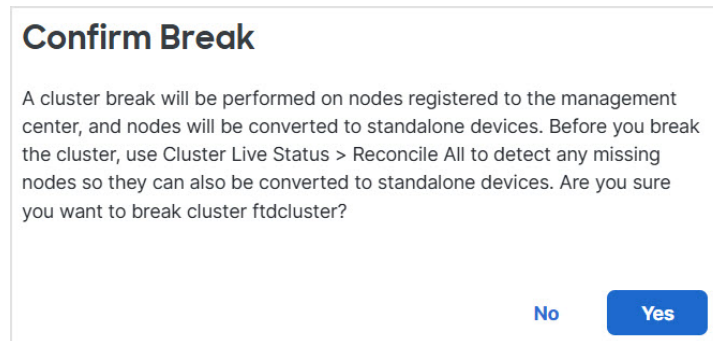
Figure 18: Confirm Break
