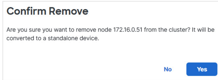
Figure 16: Confirm Break
