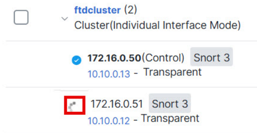
Figure 14: Node Registration
