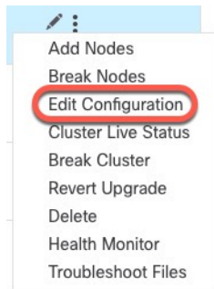
Figure 22: Edit Configuration
