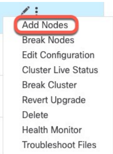
Figure 13: Add Nodes
