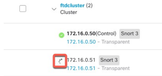
Figure 15: Node Registration
