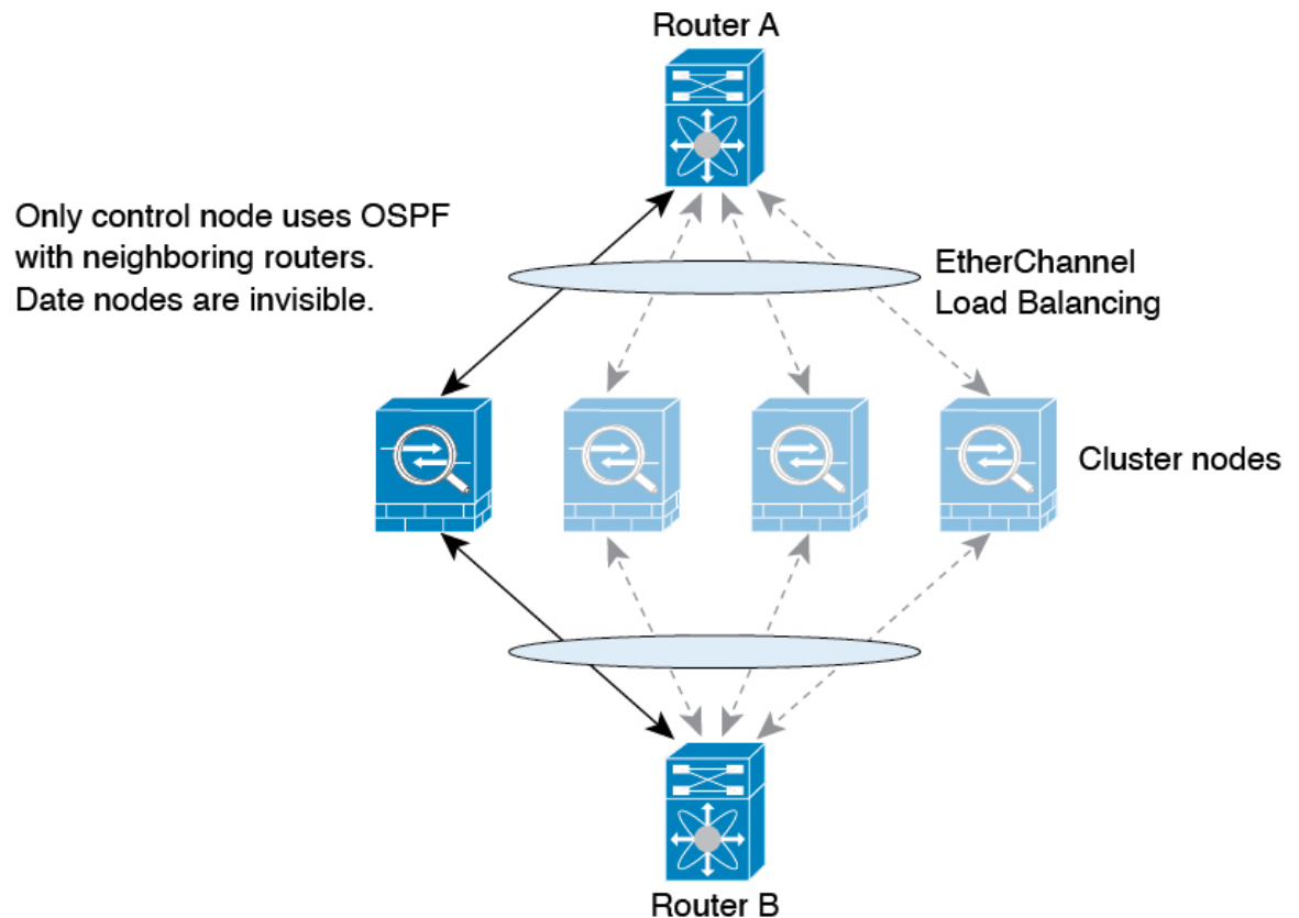
Figure 30: Dynamic Routing in Spanned EtherChannel Mode
