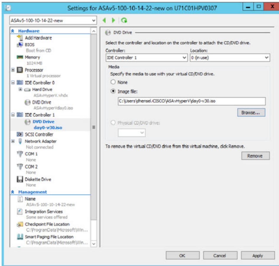
Figure 2: Hyper-V Manager
