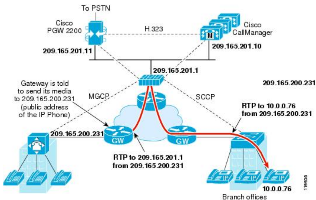
Figure 1: Using NAT with MGCP
