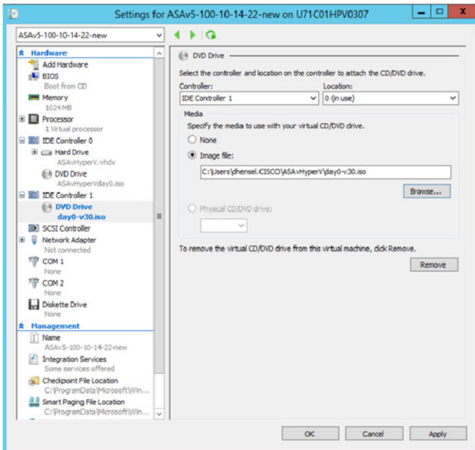
Figure 2: Hyper-V Manager
