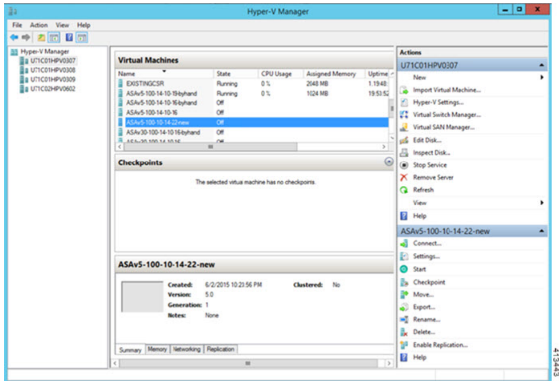
Figure 4: Hyper-V Manager
