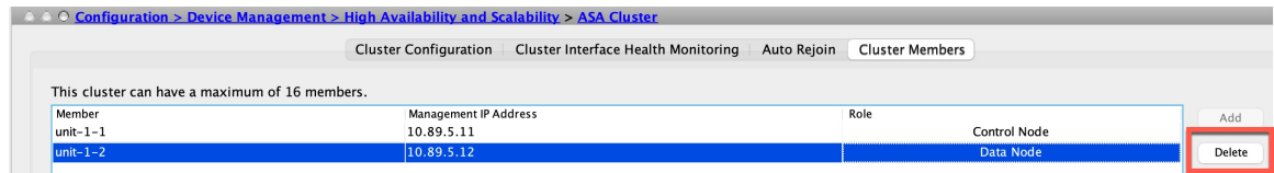
Figure 4: Delete Node
