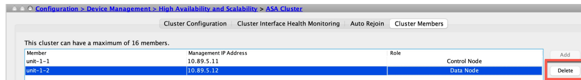
Figure 4: Delete Node
