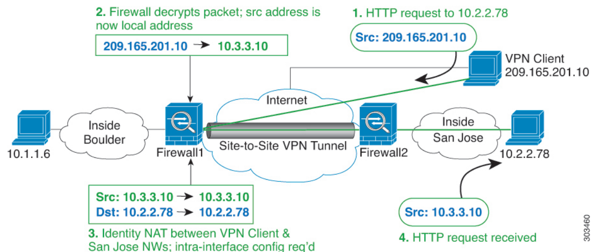
Figure 15: VPN Client Access to Site-to-Site VPN
