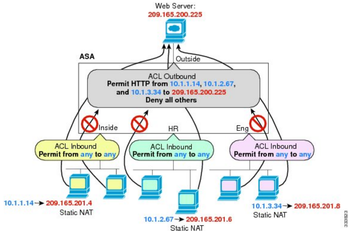
Figure 2: Outbound ACL
