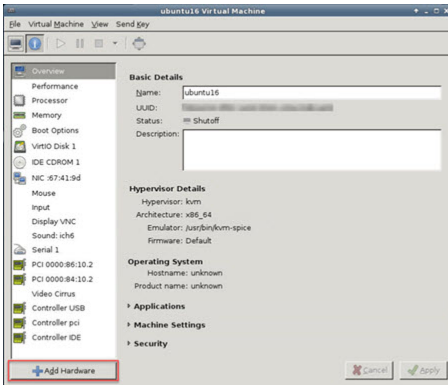
Figure 6: Add Hardware
