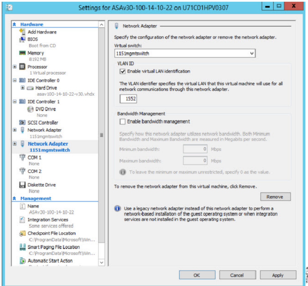
Figure 35: Modify Network Adapter Settings
