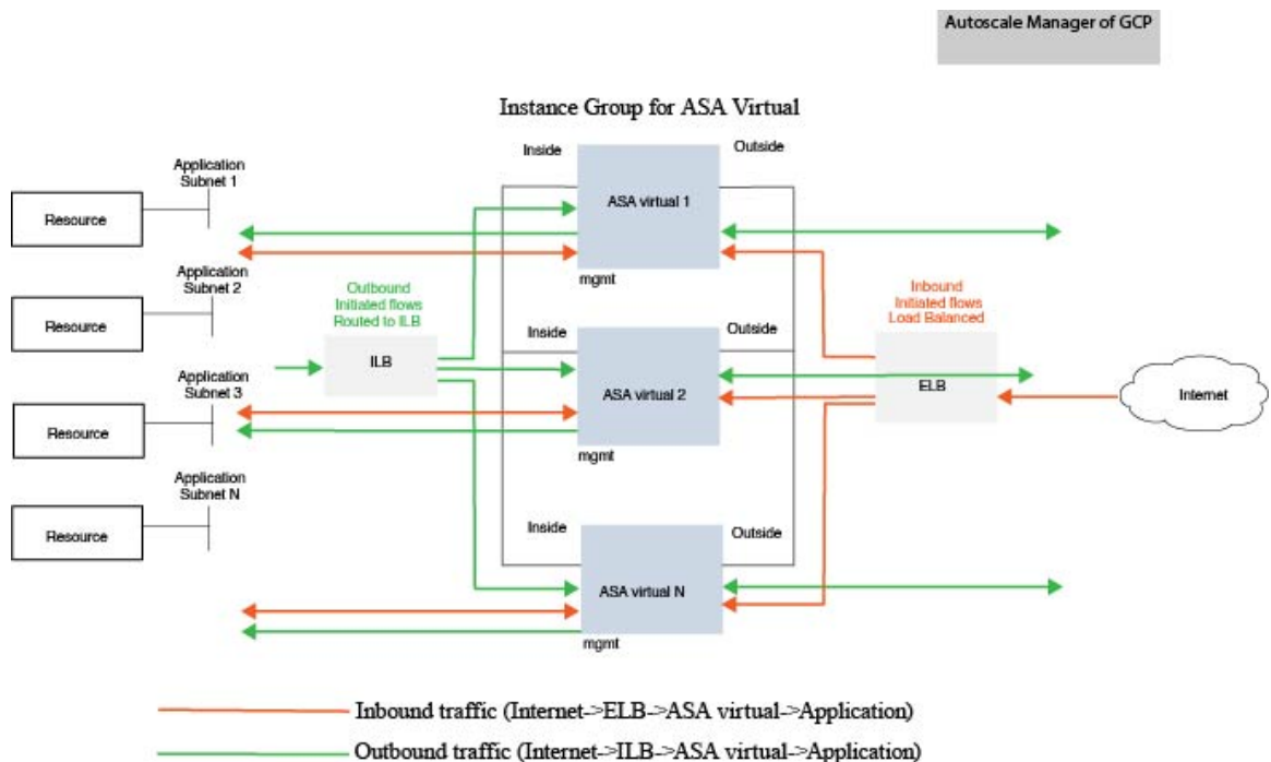
Figure 41: ASA Virtual Auto Scale Use Case
