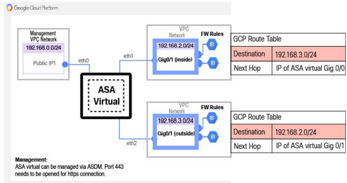
Figure 40: Sample ASA Virtual on GCP Deployment
