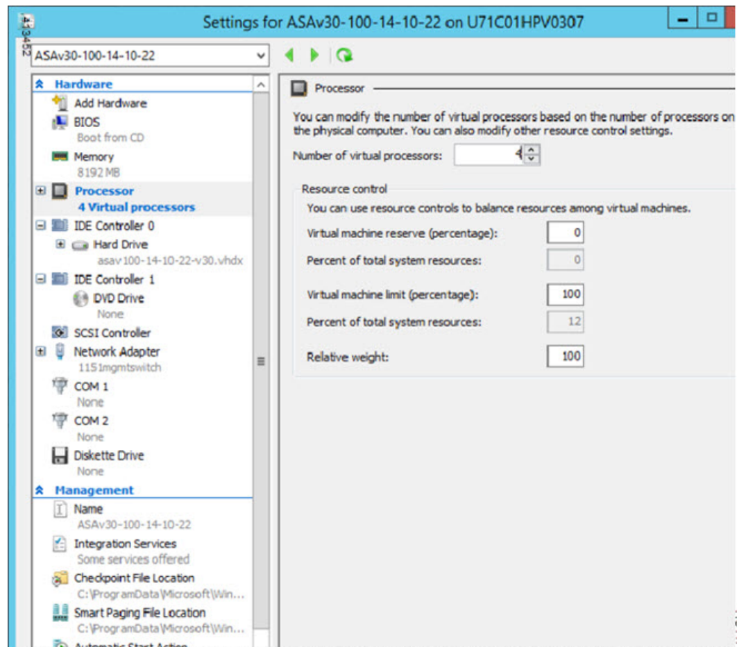
Figure 30: Virtual Machine Processor Settings
