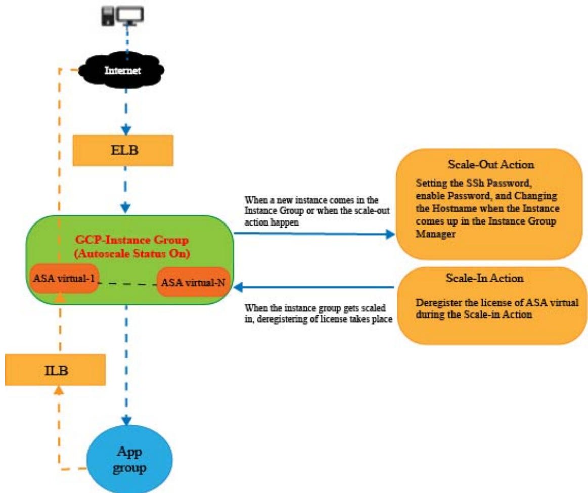
Figure 45: Autoscale Solution Overview
