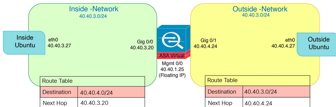
Figure 50: Sample ASA Virtual on OpenStack Deployment
