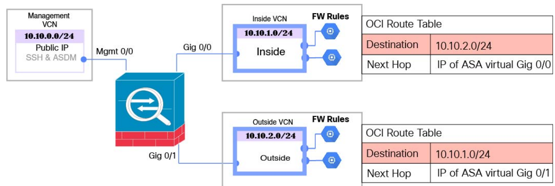
Figure 36: Sample ASA Virtual on OCI Deployment
