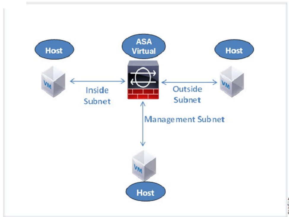
Figure 23: Recommended Topology for the ASA Virtual in Routed Firewall Mode
