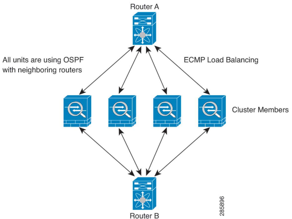
Figure 5: Dynamic Routing in Individual Interface Mode
