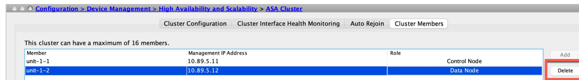
Figure 4: Delete Node
