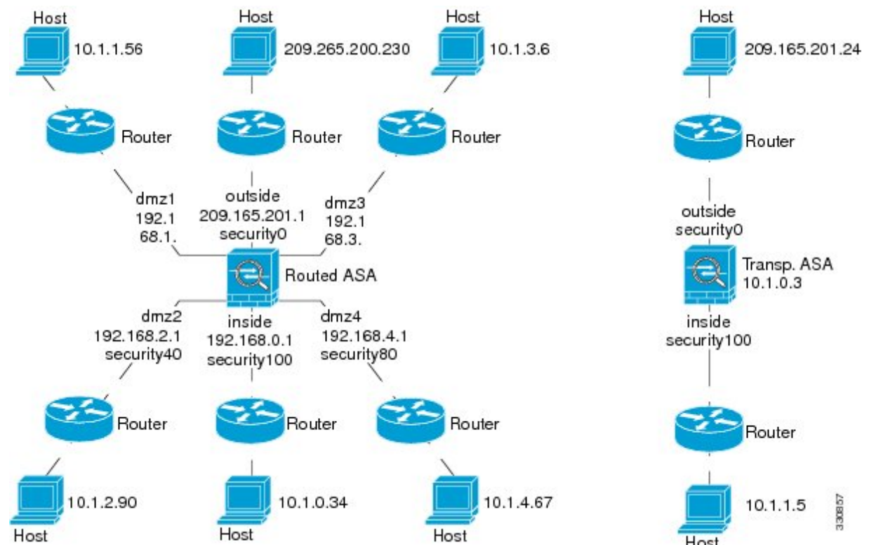
Figure 83: Network Diagram with Interfaces, Routers, and Hosts
