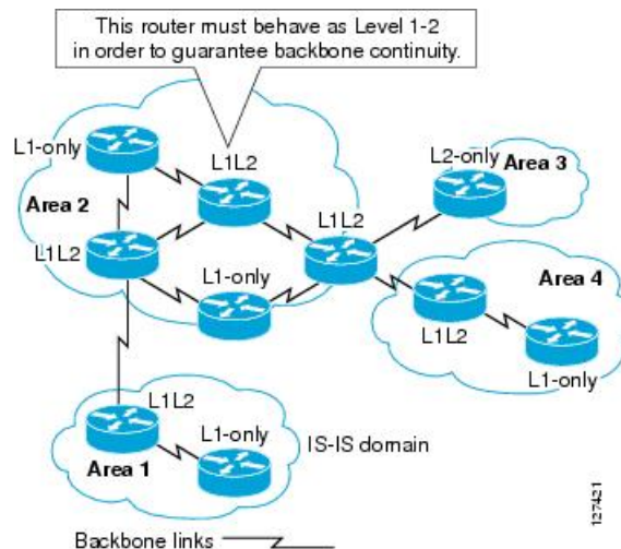
Figure 75: Level-1, Level-2, Level 1-2 Devices in an IS-IS Network Topology
