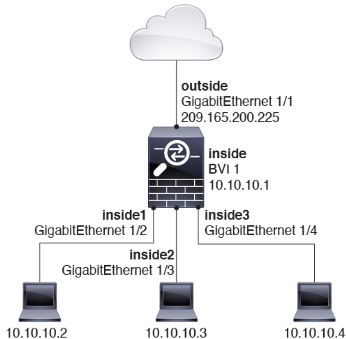
Figure 24: Routed Firewall Network with an Inside Bridge Group and an Outside Routed Interface
