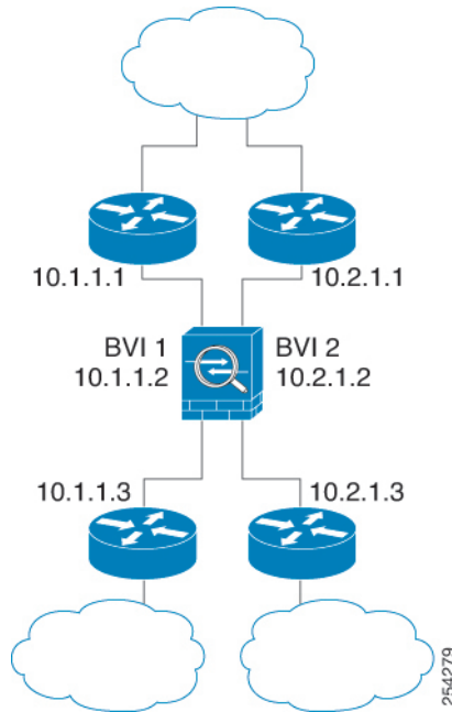
Figure 23: Transparent Firewall Network with Two Bridge Groups
