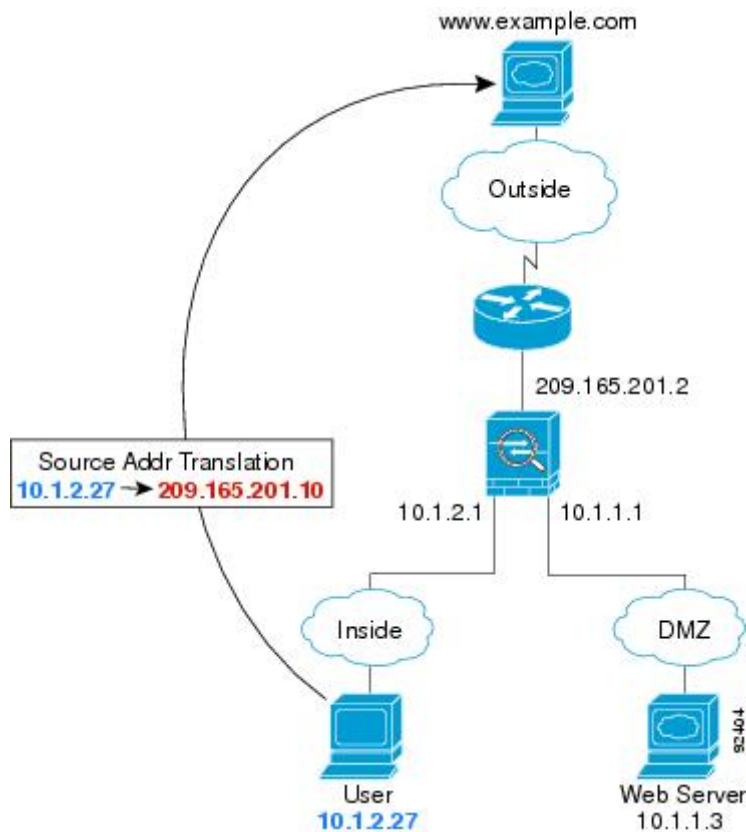
Figure 26: Inside to Outside
