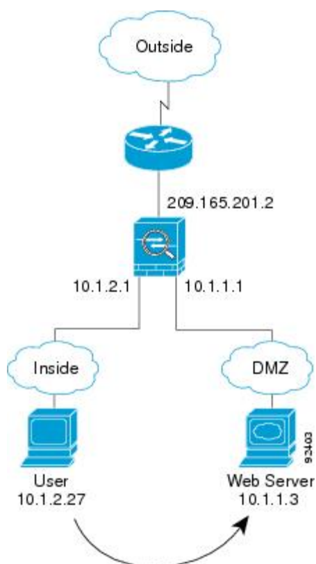
Figure 28: Inside to DMZ
