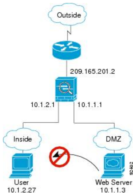
Figure 30: DMZ to Inside
