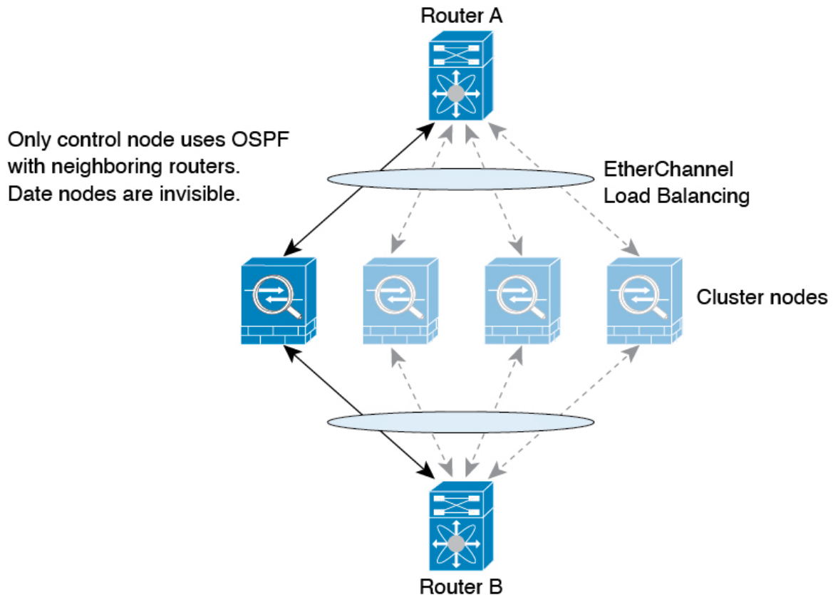
Figure 50: Dynamic Routing in Spanned EtherChannel Mode
