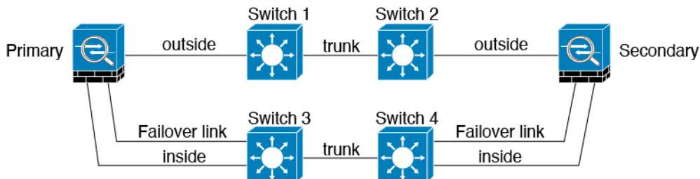
Figure 47: Connecting with a Secure Switch
