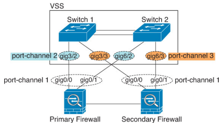
Figure 66: Active/Standby Failover and VSS/vPC
