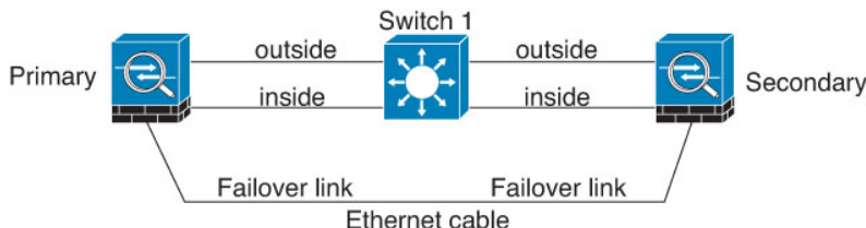
Figure 46: Connecting with a Cable
