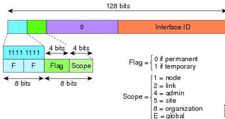
Figure 88: IPv6 Multicast Address Format
