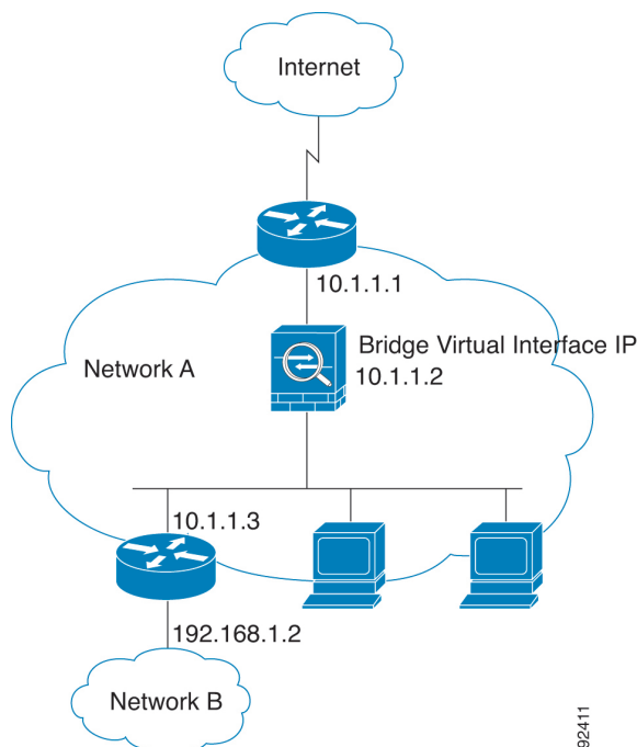
Figure 22: Transparent Firewall Network
