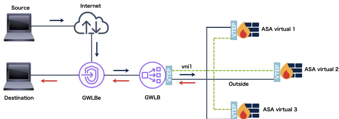
Figure 56: Geneve Single-Arm Proxy
