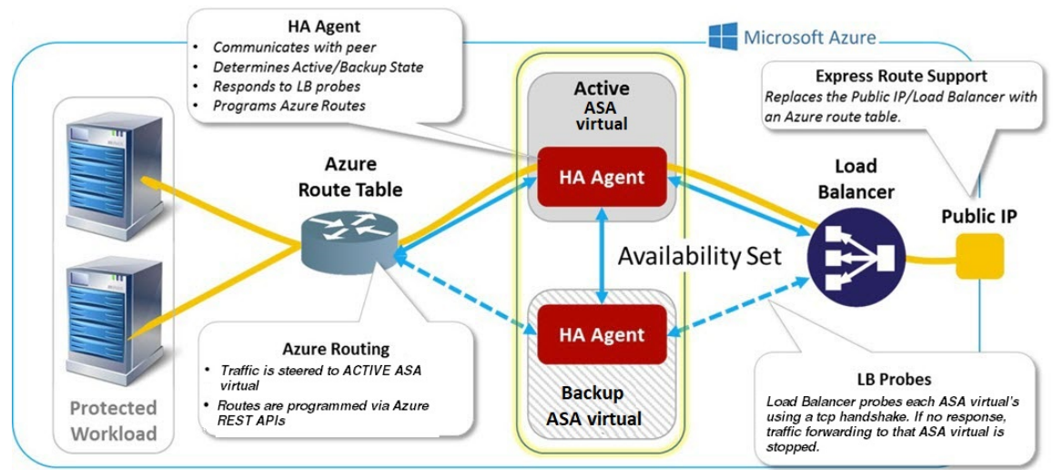
Figure 49: ASA Virtual HA Deployment in Azure
