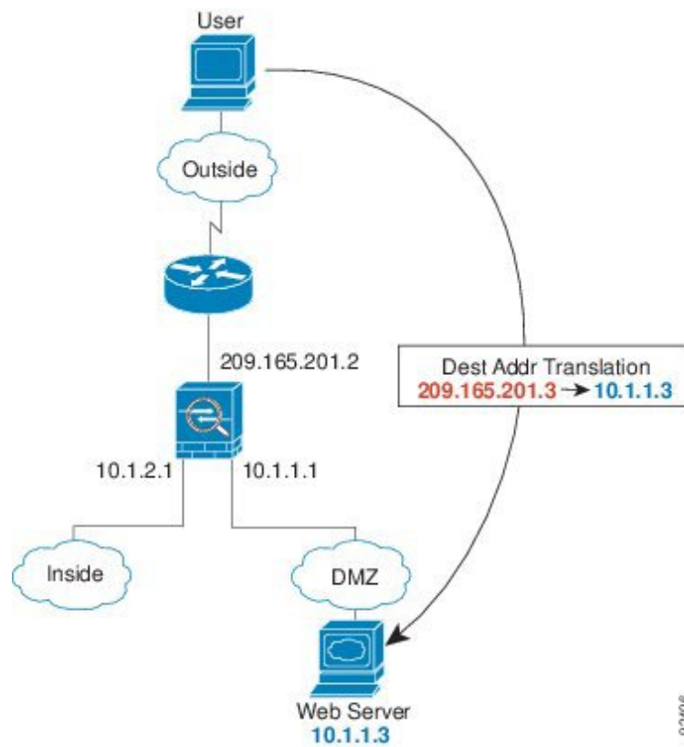
Figure 27: Outside to DMZ
