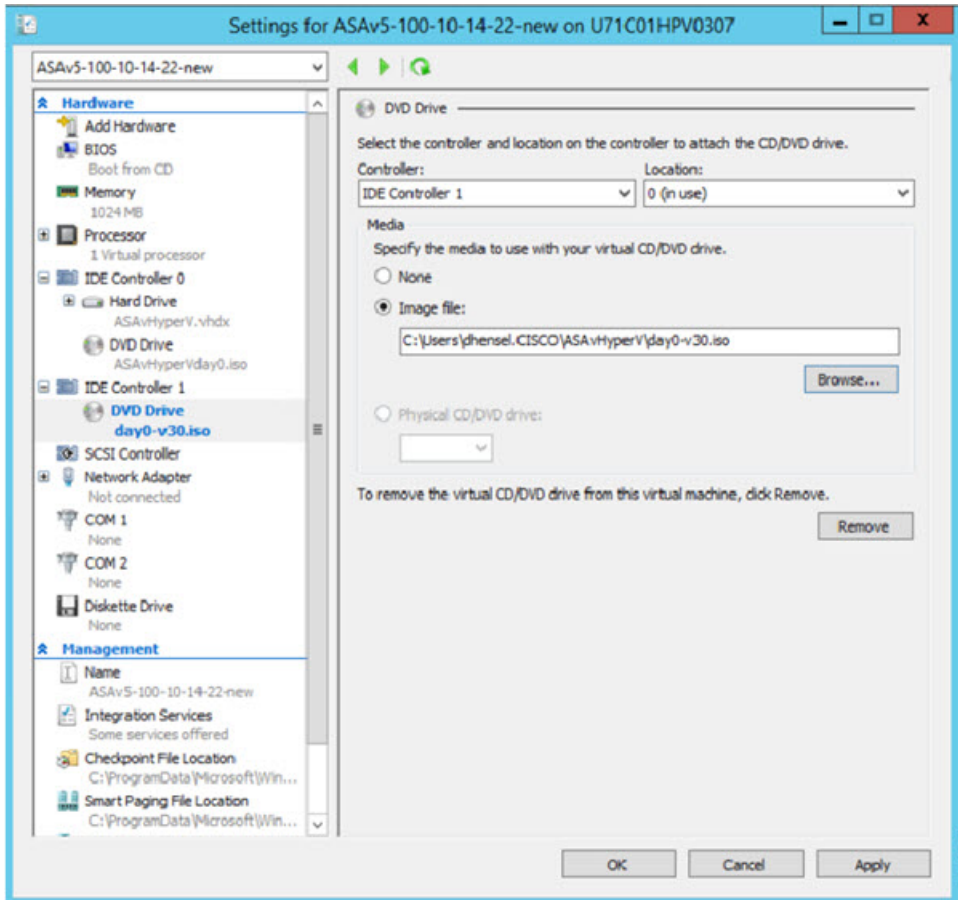
Figure 2: Hyper-V Manager
