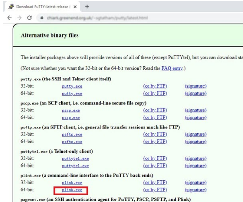
Figure 10: Download PuTTY
